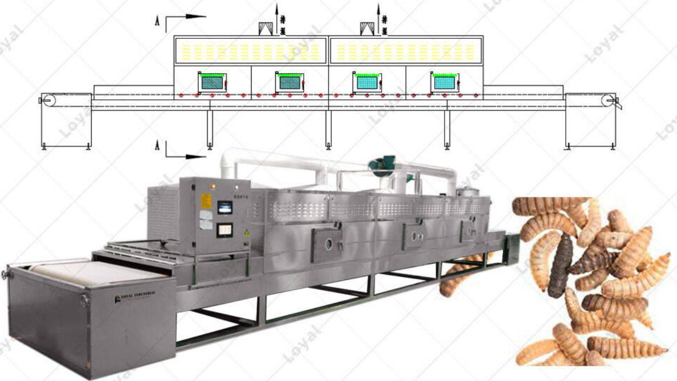
Detail of Industrial Conveyor Belt Type Microwave Oven For Black Soldier Fly Larvae Layout
