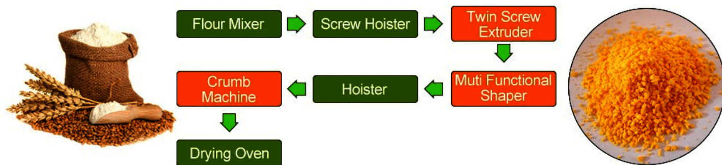
Flow Chart of Bread Crumbs Making Machine
