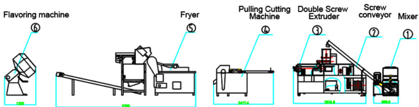
Automatic Fried Bugle Chips Production Line Layout
