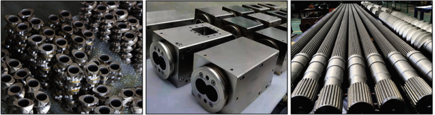
Fried Bugle Salad Chips Extruder Machine Detail Show
